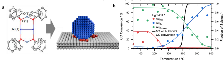
Figure 1: a) Schematic representation of the formation of Au particles stabilized by a P-containing binding pocket starting from [\text{Au}_2(\mu_2\text{-Ph}_2\text{POPPh}_2)_2]\text{OTf} [3] and b) the respective operando X-ray absorption spectroscopy measurement of the different species of gold present during the first catalytic cycle (1000 ppm CO, 10 % O 2 , balanced in N 2 , 60 000 L gAu -1 h -1 ).
